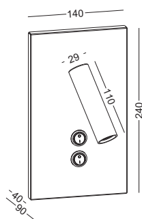
vertical installation
